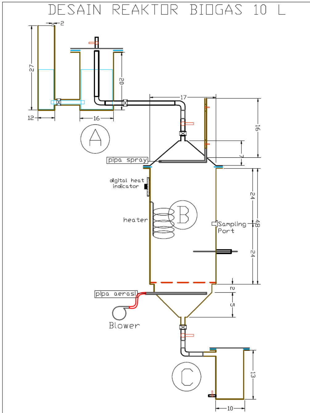
Ket : (A) Penampung gas; (B) Digester, (C) Penampung air lindi
