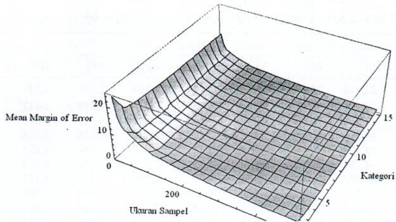
Gambar 1 Plot mean margin of error data sebaran normal \mu_1 = \mu_2 = 50, \sigma_1 = \sigma_2 = 15 .
