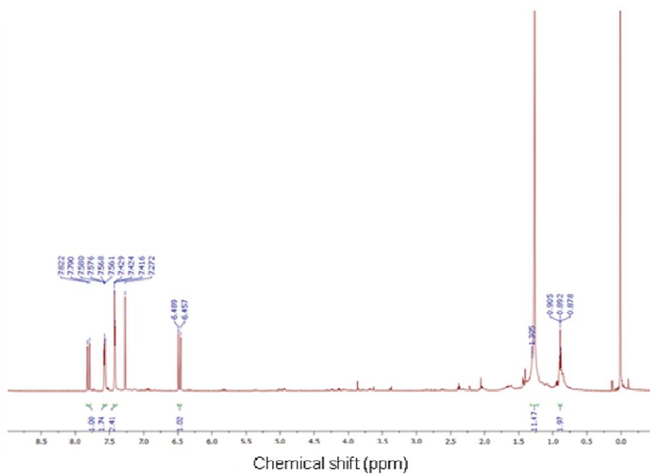
Fig. 2. ^1\text{H} NMR spectrum of \text{H}_{71} fraction (500 MHz, \text{CDCl}_3 )
