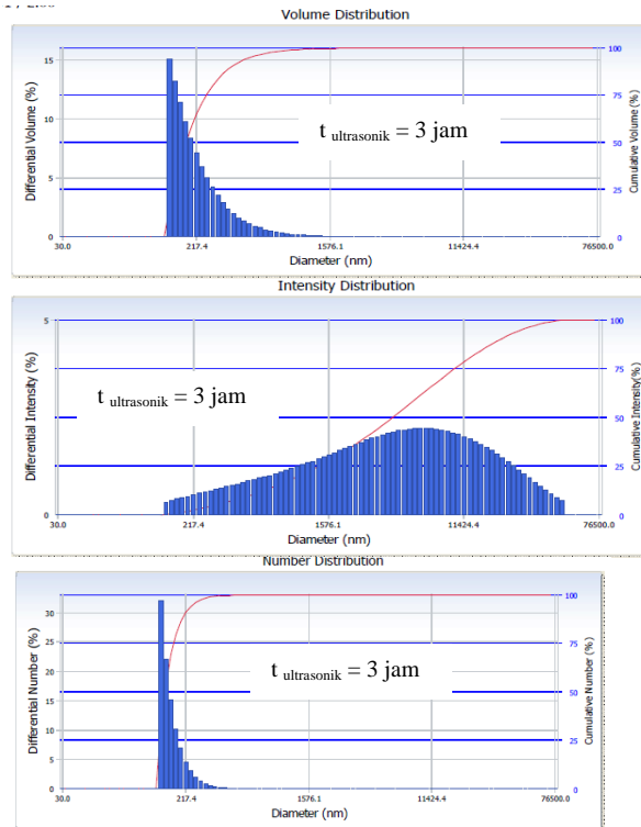
Gambar 4 Pengujian PSA, Volume, Intensity, Number Distribution (%) SKR Ultrasonik 3 jam.
