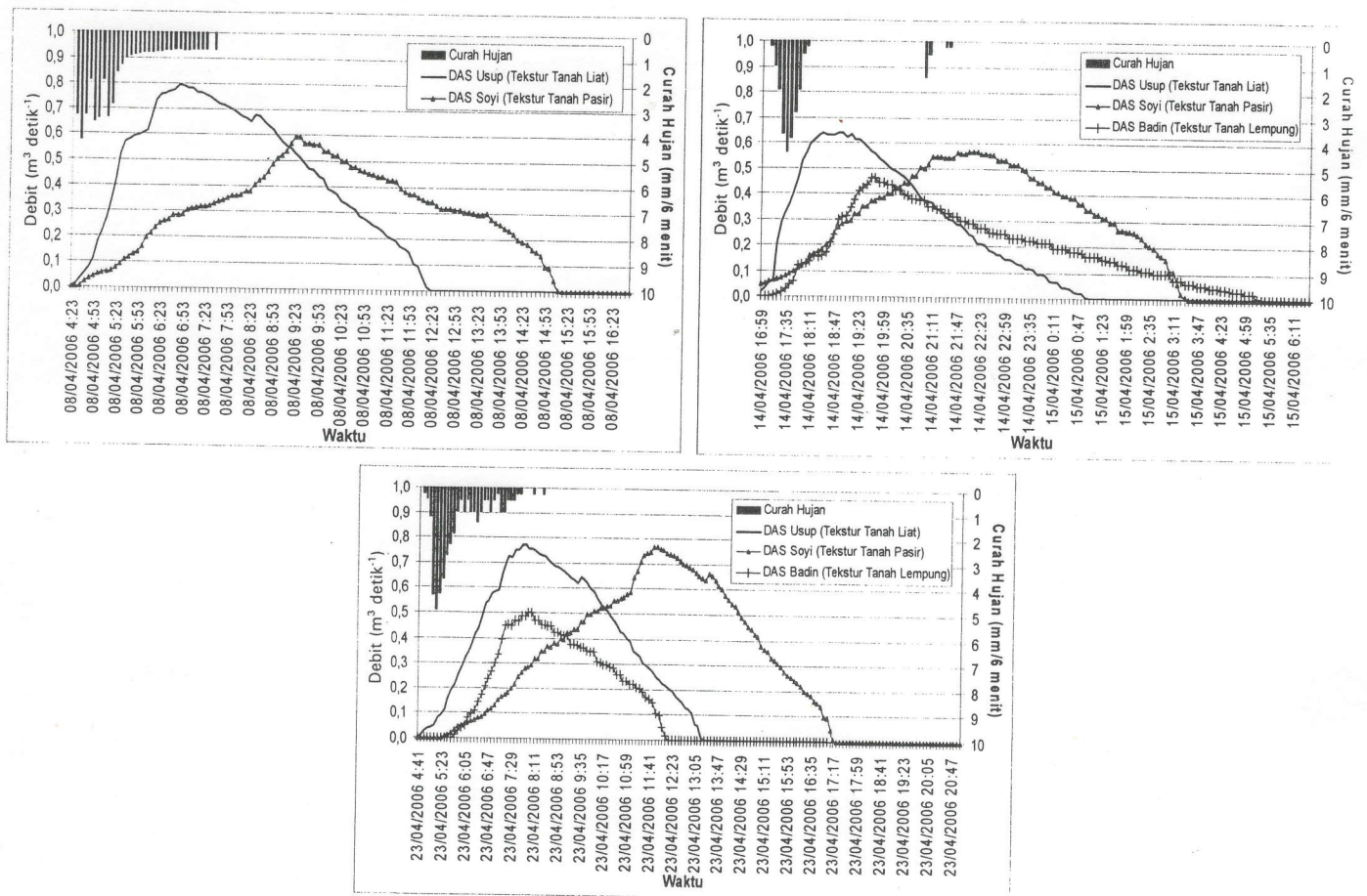
Gambar 3. Pengaruh tekstur tanah terhadap unit hidrograf Figure 3. Effect of soil texture on hydrographs unit
