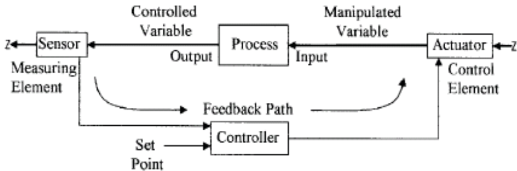
Gambar 1 Skema sistem kendali otomatis (Dunn, 2005)
