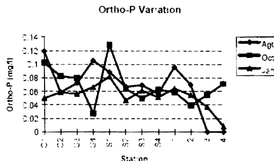
Figure 11. Orthophosphate (ortho-P) in Cimanuk river.
