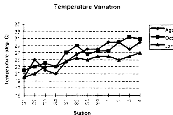
Figure 5. Temperature Variation in Cimanuk River.
