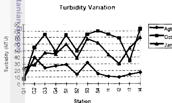
Figure 4. Turbidity Characteristics of Cimanuk River.
