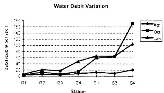
Figure 2. Flow Characteristics of Cimanuk River
