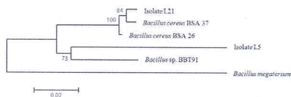
Fig. 1: Dendrogram of the chitinolytic isolates based on partial sequences of 16S rRNA gene with reference strains. The scale bar corresponds to 0.02 substitutions per nucleotide position
