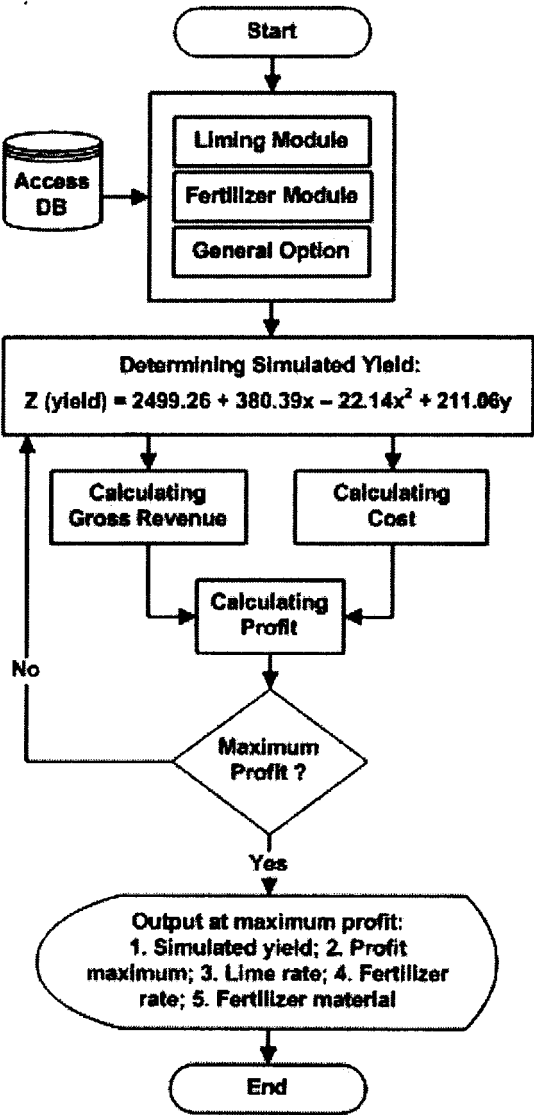
Figure 3. RiCASS Flowchart
