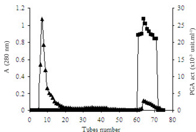
Figure 2. Elution profile of PGA activity using affinity chromatography. The column was eluted with 20 mM sodium phosphate buffer pH 6.8 and 100 mM sodium chloride. \blacktriangle : proteins and \blacksquare : PGA activity.
