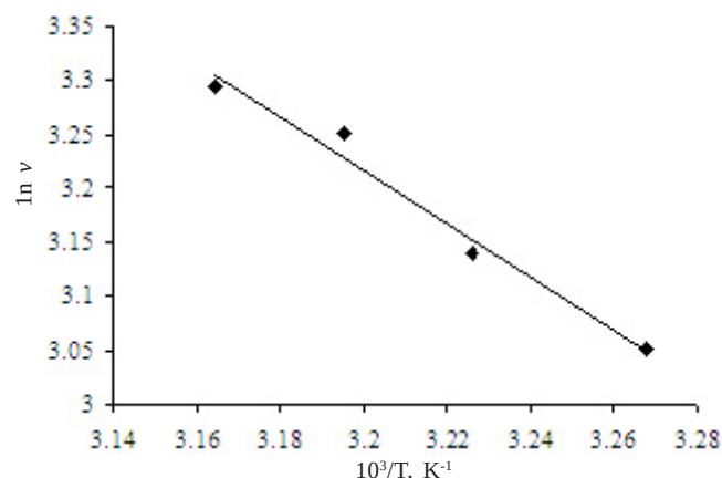
Figure 4. Arrhenius plot for determination of activation energy of extracellular B. subtilis BAC4 PGA [♦: ln v].
