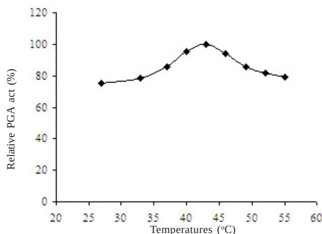
Figure 3. Effects of temperature on the PGA activity for penicillin G hydrolysis. ♦: relative PGA activity (%).
