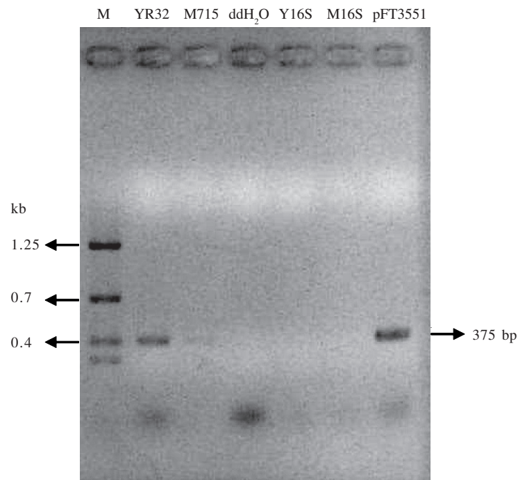
Fig 6 RT-PCR of inner membrane proteins from total RNA sample. M: Nugen Marker; YR32: Xag YR32 (RT of YR32, PCR with imps primer); M715: Mutant M715 (RT of M715, PCR with imps primer); ddH 2 O: negative control (Distillated water, PCR with imps primer); Y16S: negative control (RT of YR32, PCR with 16S rDNA primer); M16S: negative control (RT of M715, PCR with 16S rDNA primer); pFT3551: positive control (pFT3551, PCR with imps primer).
