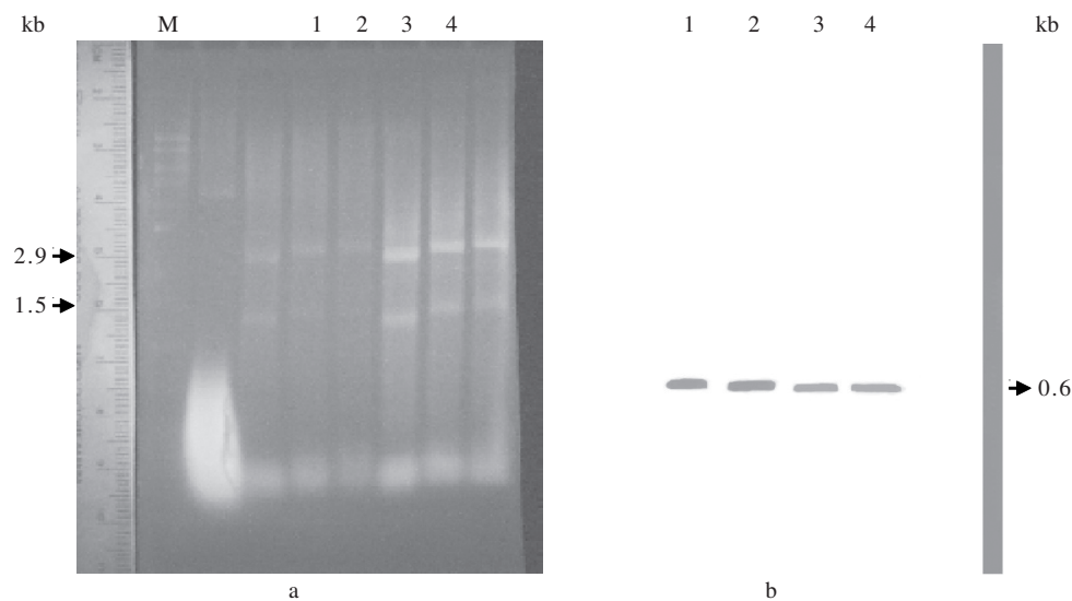
Fig 5 RNA electrophoresis and RNA-blot analysis of YR32 and M715. a. RNA electrophoregram of YR32 and M715, b. RNA-blot of YR32 and M715 with inner membrane proteins probe. Lane 1 and 2: YR32, lane 3 and 4: M715; lane M: 1 kb DNA ladder (New England Biolabs, Beverly, USA).
