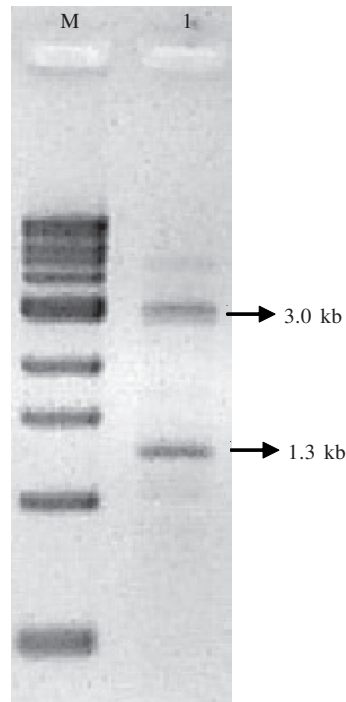
Fig 1 Agarose gel electrophoresis profile of IPCR product. M: 1 kb DNA ladder (New England Biolabs, Beverly, USA). 1: IPCR.
