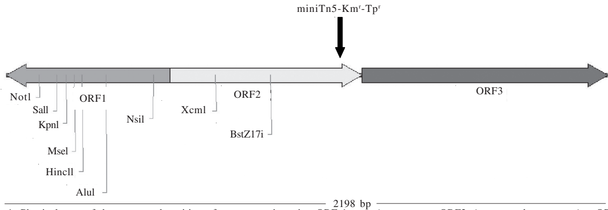
Fig 4 Physical map of the genes and position of transposon insertion ORF 1: cystein proteases , ORF2: inner membrane proteins , ORF3: TonB dependent-receptor .
