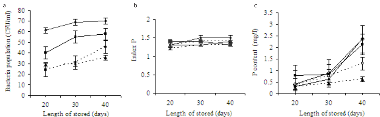
Figure 2. Relationship between population of bacteria (a) and Soluble P Index (b), with the content of P-available (c) in the compost extracts. A and B were the total numbers of bacteria grown on the Pikovskaya medium. C: compost of vegetable wastes, +E or -E = amended with or without EM4, +B or -B = amended with or without P. aeruginosa Ch1, [C+E+B] directly = Organic material amended with EM4 and P. aeruginosa Ch1 directly at the same times, composted then extracted. \triangle —: C-E-B; \square —: C-E-B+; \circ —: (C+E+B) directly; \bullet —: C-E+B+; \blacksquare —: C+E+B
