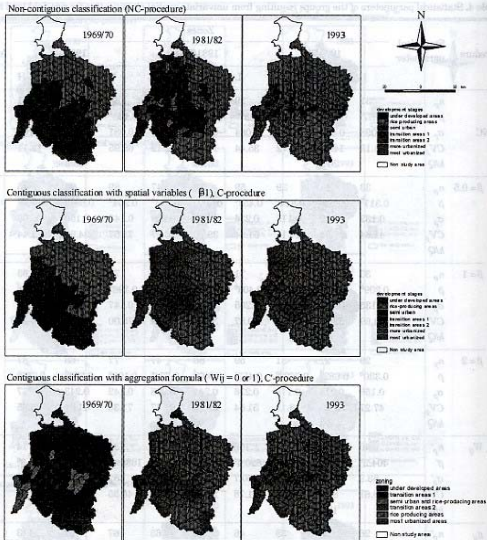
Fig. 6. Multivariate classification
