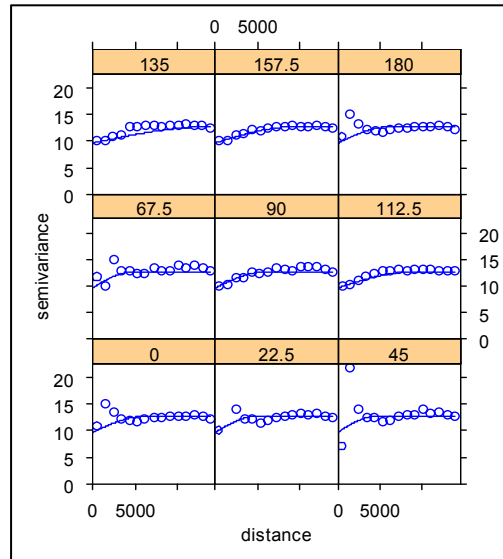
Figure 5. The directional variograms of the stand volume
