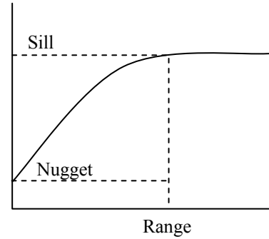
Figure 2. A theoretical variogram
