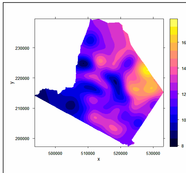
Figure 7. Prediction map of the stand volume obtained from the universal kriging (not to scale). The values are squared-root of stand volume in \text{m}^3/\text{ha} .
