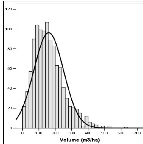
Figure 3. Distribution of the stand volume
