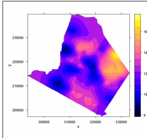
Figure 6. Prediction map of the stand volume obtained from the ordinary kriging (not to scale). The values are squared-root of stand volume in \text{m}^3/\text{ha} .
