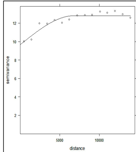
Figure 4. The spherical variogram of the stand volume
