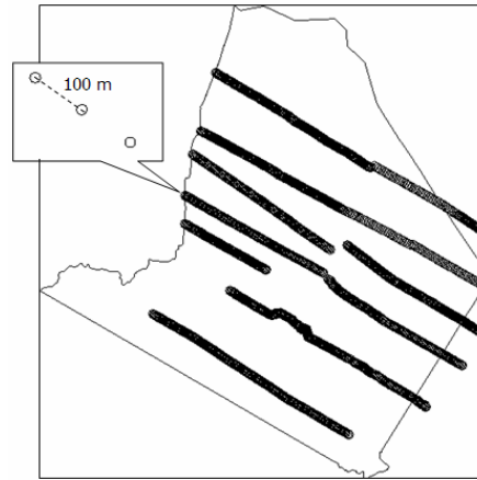
Figure 1. Layout of the sample plots in the study area
