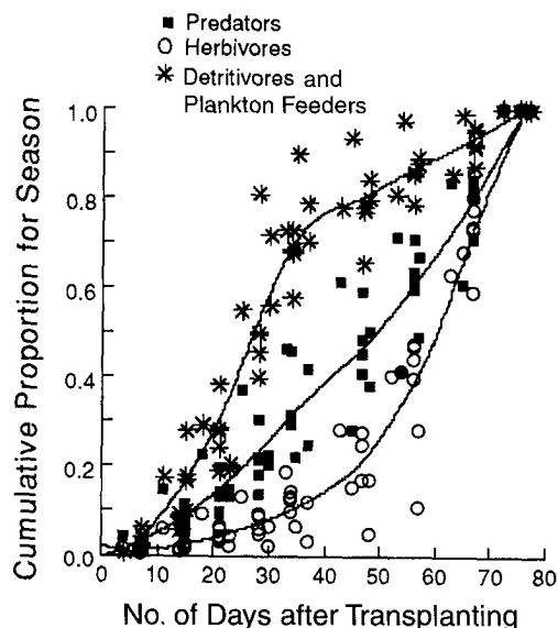
FIG 2. The cumulative proportion of total seasonal abundance of three trophic levels over one season, compiled from six locations in Java. Curves represent Loess fits, tension = 0.5. Note that populations of detritivores and plankton feeders emerge earliest, followed by predators, and finally by herbivores. This supports the hypothesis that predators are feeding on populations of detritivores and plankton feeders.
