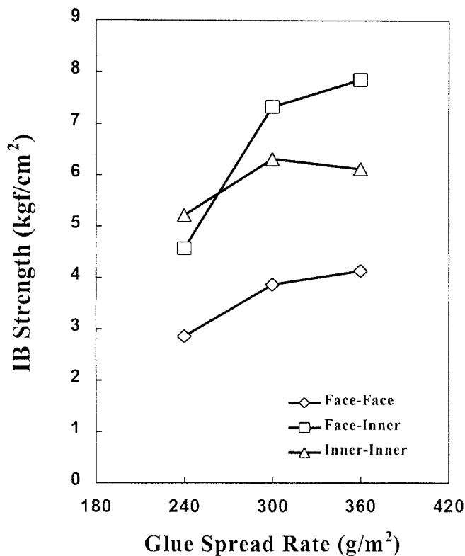
Fig. 4. Internal bond strength (IB) of two-ply LBL at different glue spread rates. Diamonds, glue spread rate on face-to-face layer; squares, glue spread rate on face to inner layer; triangles, glue spread rate on inner to inner layer
