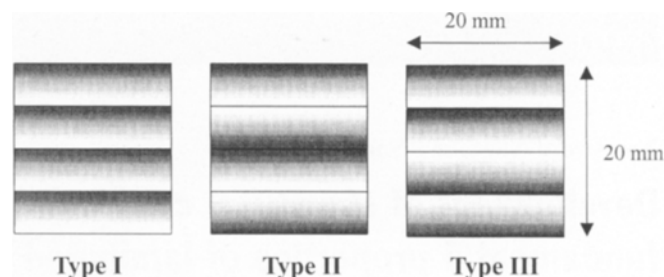
Fig. 2. Combination of layered structure on laminated bamboo lumber (LBL). Light color, inner layer; dark color, face layer
