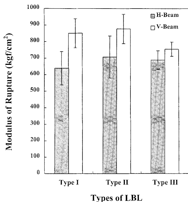
Fig. 6. Modulus of rupture of LBL according to the bending test position. Shaded bars (H-beam), load applied to the specimens with horizontal glue line; open bars (V-beam), load applied to the specimens with vertical glue line. Each vertical bar indicates the standard deviation
