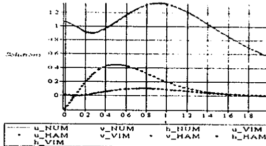
Figure 1 NUM, HAM and VIM solutions u(x, t) , v(x, t) , h(x, t) , for t = 0.1 and 0 \leq x \leq 2 .
