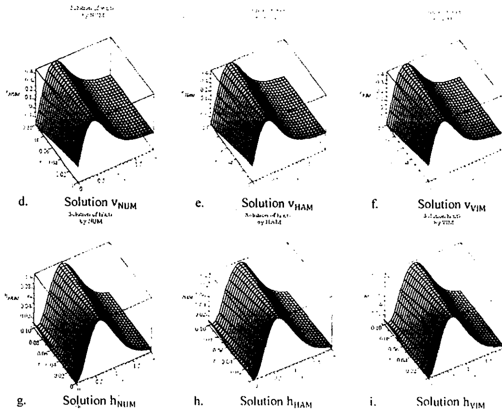
Figure 3 NUM, HAM and VIM solutions u(x, t) , v(x, t) , h(x, t) , for 0 \leq x \leq 2 and 0 \leq t \leq 0.1 .
