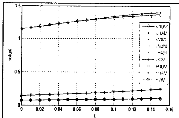
Figure 2 NUM, HAM and VIM solutions u(x, t) , v(x, t) , h(x, t) , for x = 1 and 0 \leq t \leq 0.15 .
