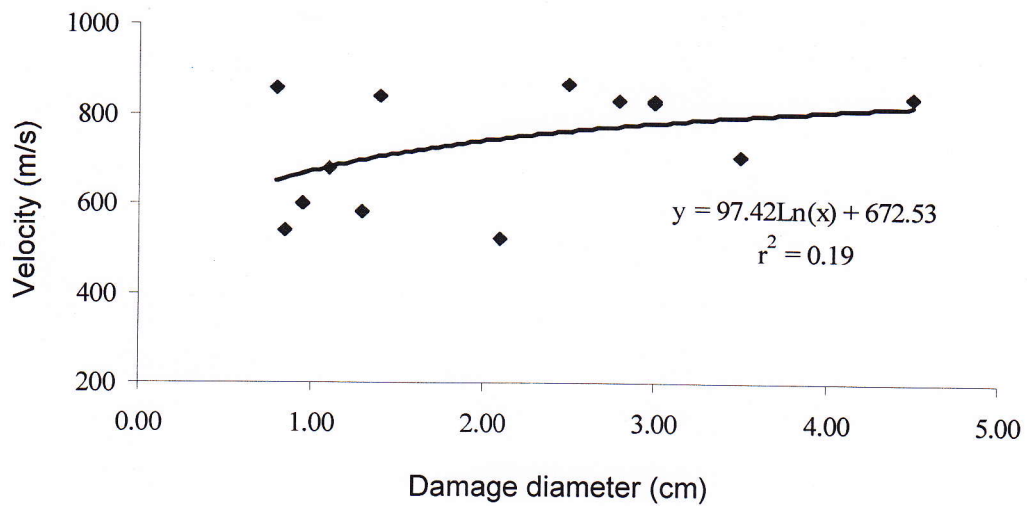
Figure 9. Correlation between ultrasonic wave velocity and damage diameter
