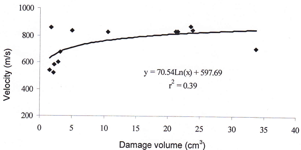
Figure 6. Correlation between damage volume and velocity
