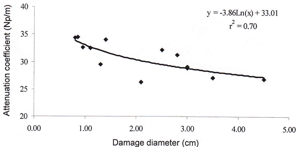
Figure 8. Correlation between attenuation coefficient and damage diameter
