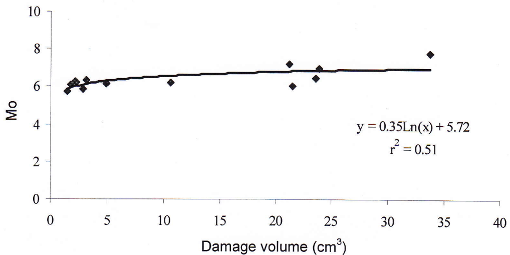
Figure 7. Correlation between damage volume and moment zero power
