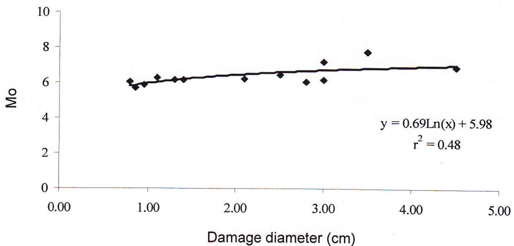
Figure 10. Correlation between zero moment power and damage diameter
