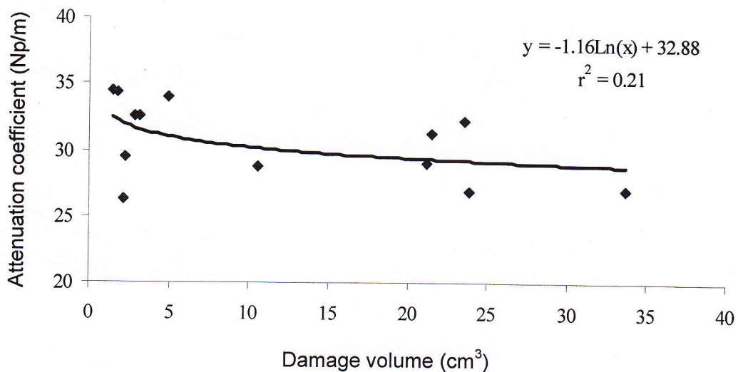
Figure 5. Correlation between damage volume and ultrasonic coefficient.
