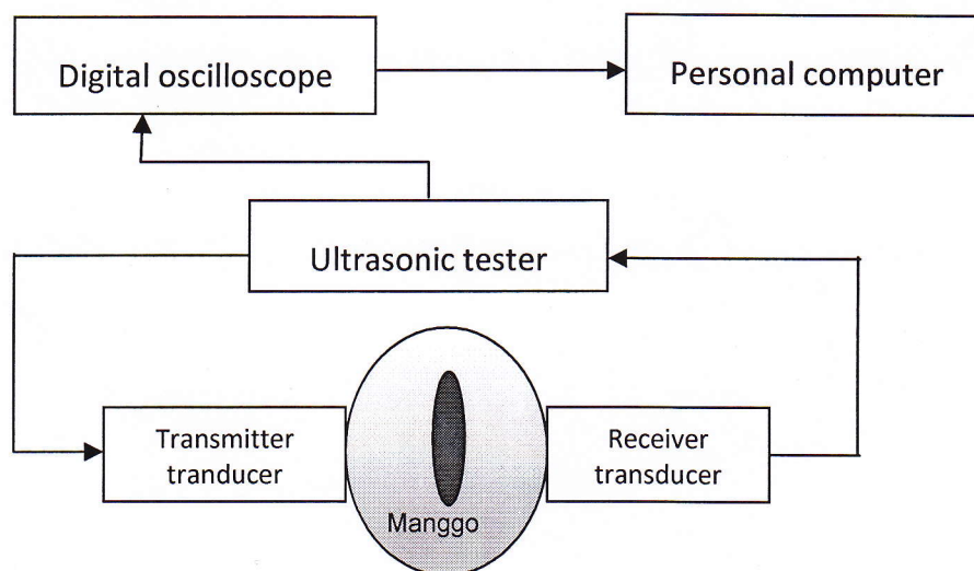
Figure 1. ultrasonic measurement.
