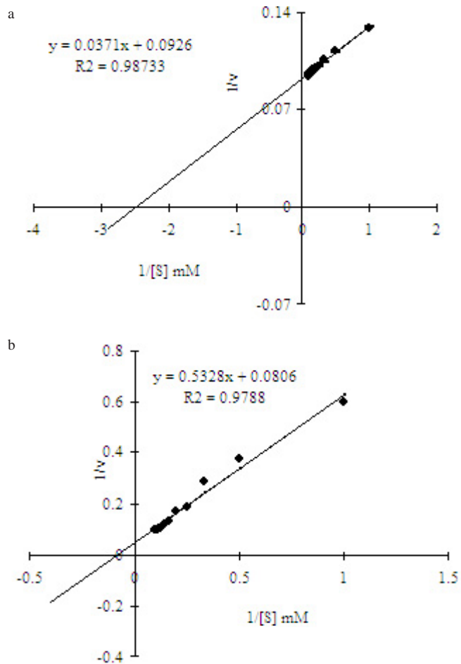
Figure 5. Lineweaver-Burk plot for (a) tannic acid, (b) gallotannin.
