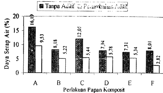
Gambar 3. Histogram daya serap air 24 jam
