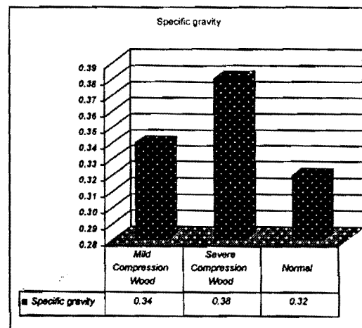
Fig 6. Comparison of SG between compression wood and normal wood.
