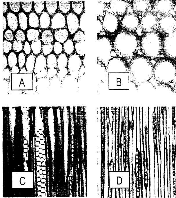
Figure 1 A. Cross section of tracheid cells of normal wood of Agathis, has a rectangular form. B. Cross section of tracheid cells of Agathis compression wood, has a round form and has intracellular space. C. Bordered pits alternate distribution on radial wall of tracheid cells of Agathis. D. Ray cells orientation ( uniseriate ) on tangential wall of tracheid cells of Agathis.
