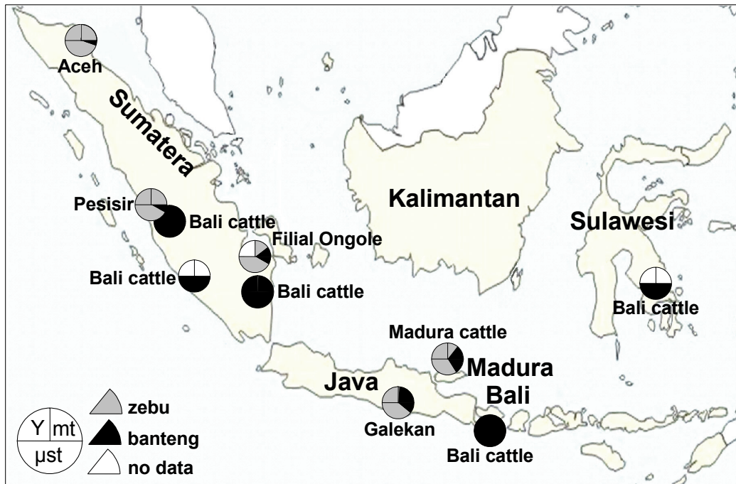
Figure 1. Locations of sampling and genetic constitution of Indonesian cattle populations. The species origin of the paternally transmitted Y-chromosomes (Y), maternally transmitted mitochondrial DNA (mt) and autosomal microsatellite alleles ( \mu st) is represented by black and gray shading of the indicated circle segments.
