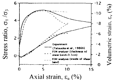
Figure 3. Simulated stress-strain volume of triaxial test
