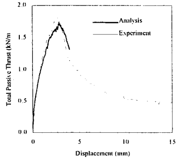
Figure 7. Analytical and experimental result for Toyoura sand
