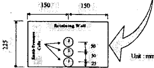
(c) Location of the earth pressure cells
