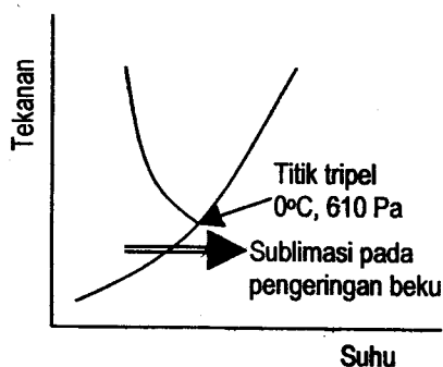
Gambar 1. Diagram P-T air
