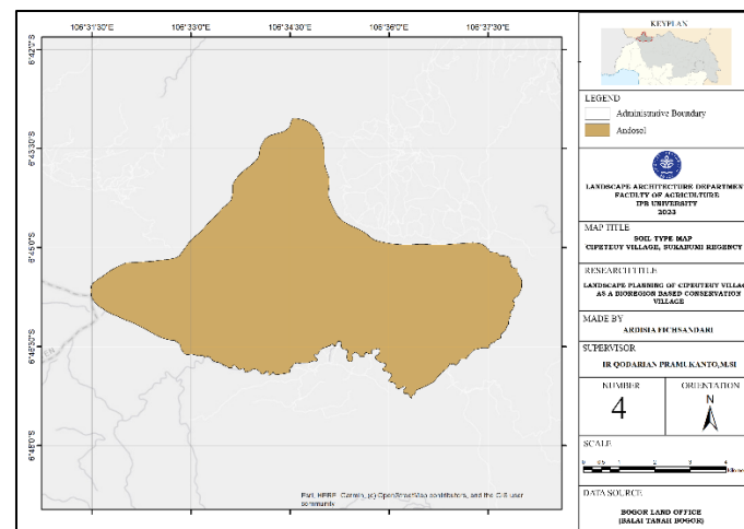
Figure 4. Soil Type Map
