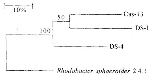
Figure 2. Phylogenetic tree of MFLP profiles generated from total genomic DNA digested with AseI . The number at the tree lines represented bootstrap values.
