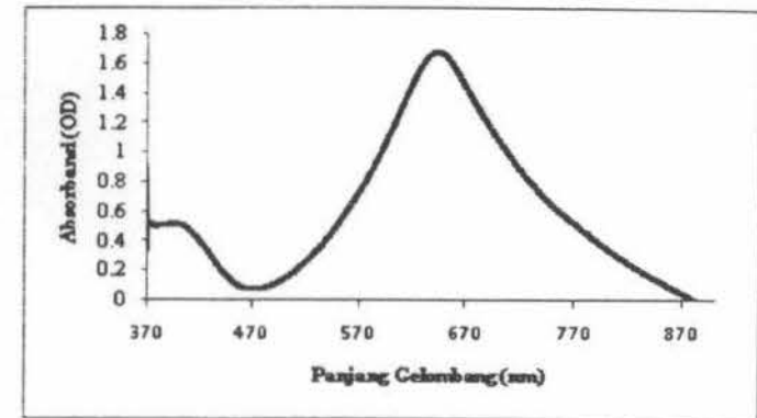
Gambar 5 Absorbansi film PANI
