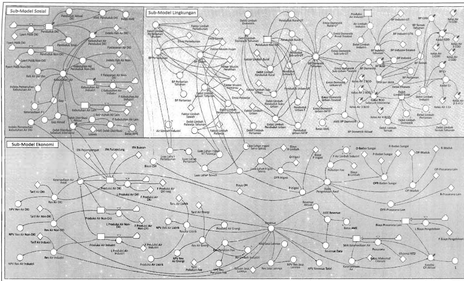
Gambar 4 Stock-flow diagram model pengelolaan sumber daya air DAS Citarum
