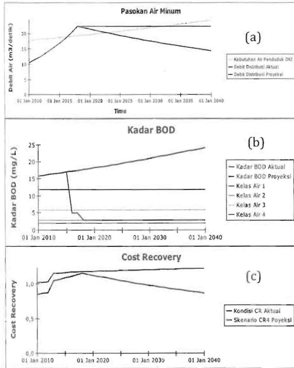
Gambar 5 Hasil simulasi model pengelolaan SDA Citarum: (a) dinamika pasokan air, (b) dinamika beban pencemaran, (c) dinamika cost recovery .
