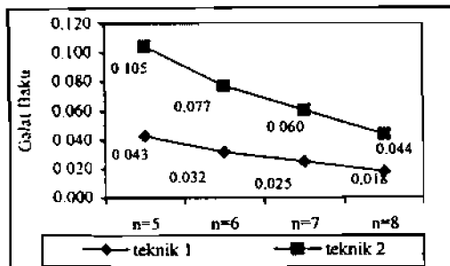
Gambar 4. Rataan galat baku penduga \mu
