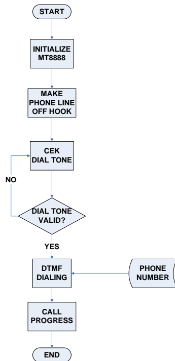
Gambar 4 Diagram alir proses dial up .
