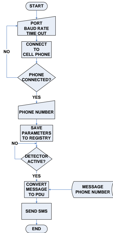
Gambar 5 Diagram alir proses pengiriman SMS.
