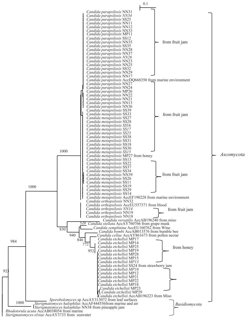
Fig 2 Dendrogram showing the phylogenetic relationship of Candida parapsilosis and C. etchellsii isolates from jam and honey with related yeast species based on ITS region. Bootstrap values, expressed as percentages of 1000 replications, are given at branch points (only values >50% are shown).
