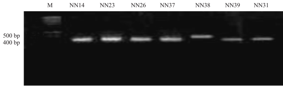
Fig 1 Gel electrophoresis images showing PCR products of yeast ITS region rDNA (about 400-500 bp in size). M, Marker; NN14, NN23, NN26, NN27, NN38, NN39, NN31, isolate from pineapple jam.
