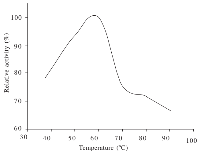
Fig 6 Effect of temperature on xylanase activity at pH 7.0.
