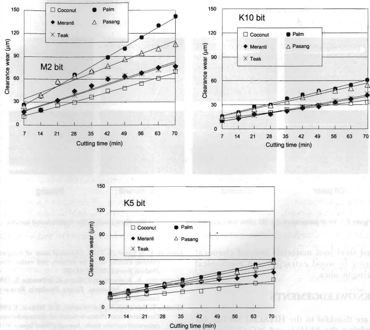
Figure 2 Clearance face wear of the bits as a function of cutting time for routing some tropical woods
