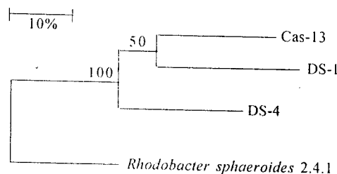
Figure 2. Phylogenetic tree of MFLP profiles generated from total genomic DNA digested with AseI . The number at the tree lines represented bootstrap values.
