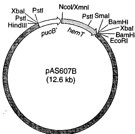
Fig. 1 Restriction map of recombinant plasmid carrying pucB'-hemT translational fusion
