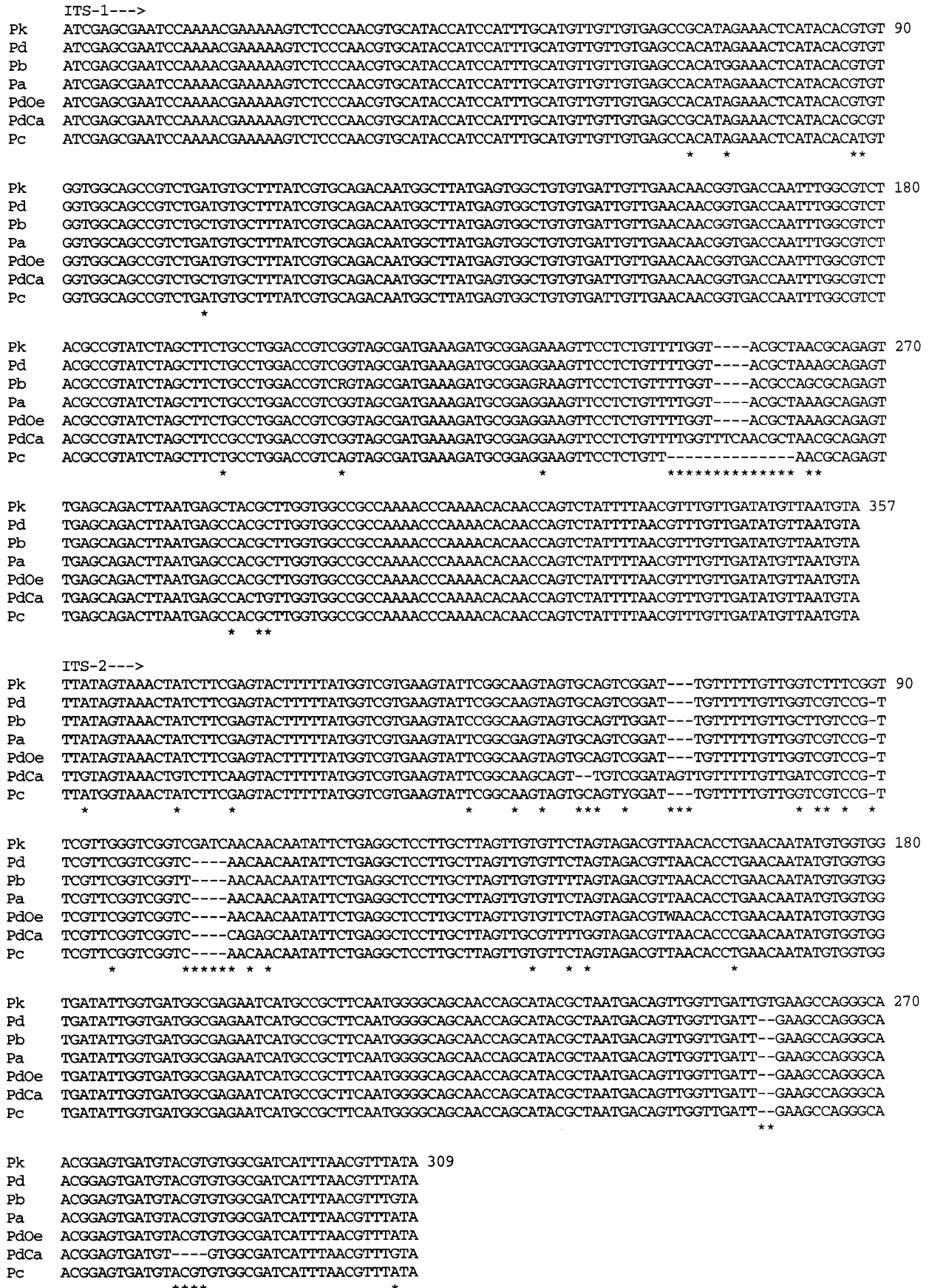
Fig. 2. Alignment of the ITS-1 and ITS-2 sequences representing Pseudoterranova krabbei (Pk), P. decipiens (s.s.) (Pd), P. bulbosa (Pb), P. azarasi (Pa) and P. decipiens (s.l.) from Osmerus eperlanus (PdOe) or Chaenocephalus aceratus (PdCa) as well as those of P. cattani (Pc). Refer to Tables 1 and 2 for samples sequenced. Sequences have been deposited in the EMBL, GenBank™ and DDBJ databases. Nucleotide differences among the aligned sequences are indicated by asterisks. Polymorphic sites in the sequences are designated with IUPAC codes.
