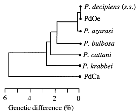
Fig. 3. Phenogram depicting the genetic differences (upon pairwise comparison) among Pseudoterranova krabbei , P. decipiens ( s.s. ), P. bulbosa , P. azarasi , P. cattani and P. decipiens ( s.l. ) from Chaenocephalus aceratus (PdCa) or Osmerus eperlanus (PdOe) for the entire ITS rDNA sequence.
