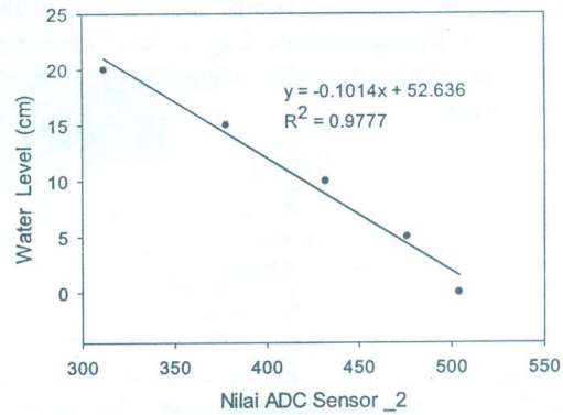
Gambar 6 Kurva Kalibrasi Sensor Water Level 1
