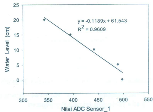
Gambar 7 Kurva Kalibrasi Sensor Water Level 2
