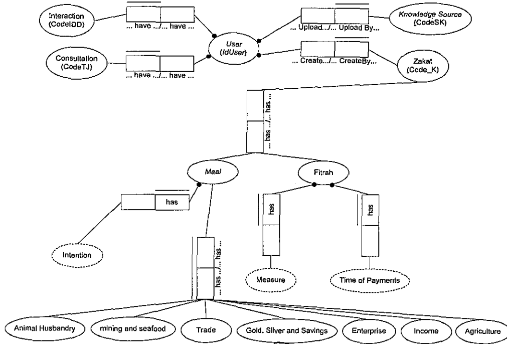
Figure 6. ORM of ZKMS
