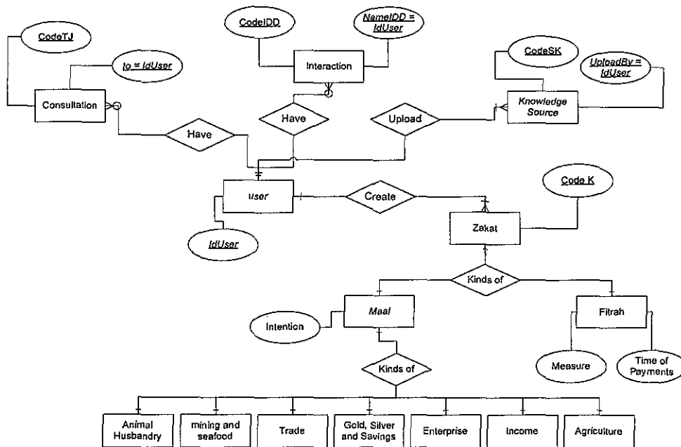
Figure 7. ERD of ZKMS
