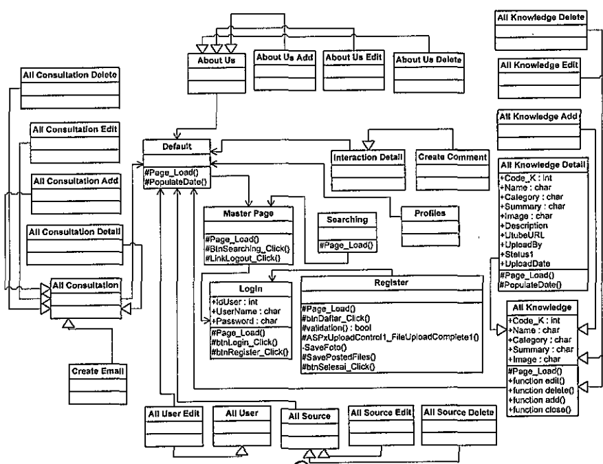
Figure 5. ClassDiagram of ZKMS
