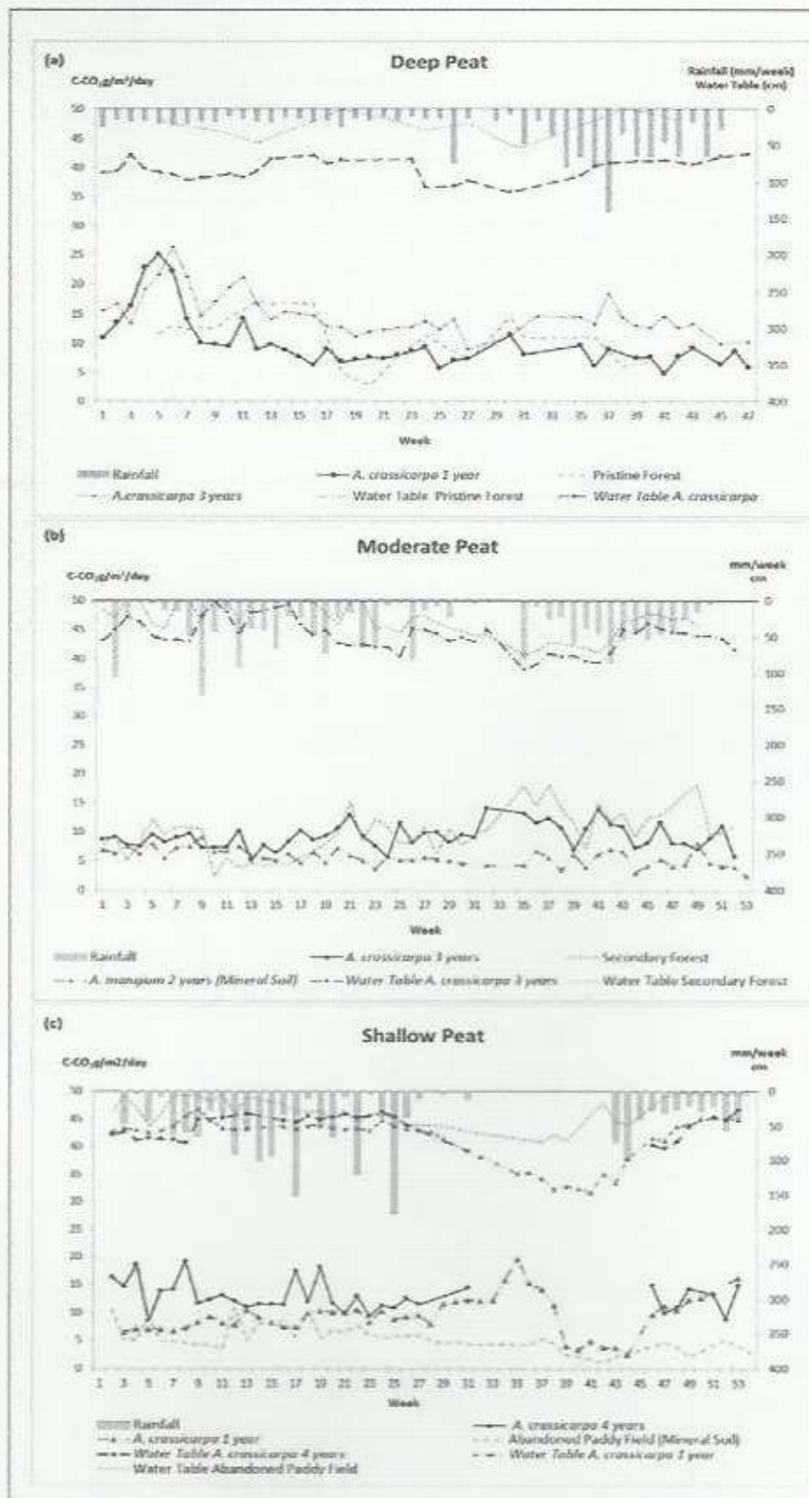
Figure 1. Weekly fluxes of CO 2 from various conditions of Acacia crassiorpa planted peatlands and from adjacent pristine forest and mineral soils.
