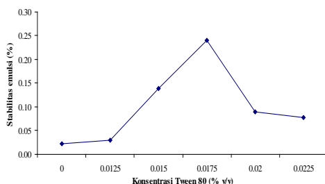
Gambar 3 Stabilitas emulsi Tween 80.
