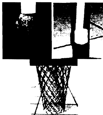
Figure 1. Anode materials used for the Biorock experiment ( left : Aluminum, middle : Magnesium, right : Titanium)
