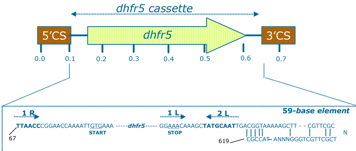
Figure 3 Characterization of gene cassette structure ( dhfr5 ) which is integrated in the class 1 integron FC12A. Open Reading Frame dhfr5 gene was shown in box. Start and stop translation codon were underlined. Putative 59 be region, 1R, 1L, and 2L for integrase binding domains were shown with arrows.
