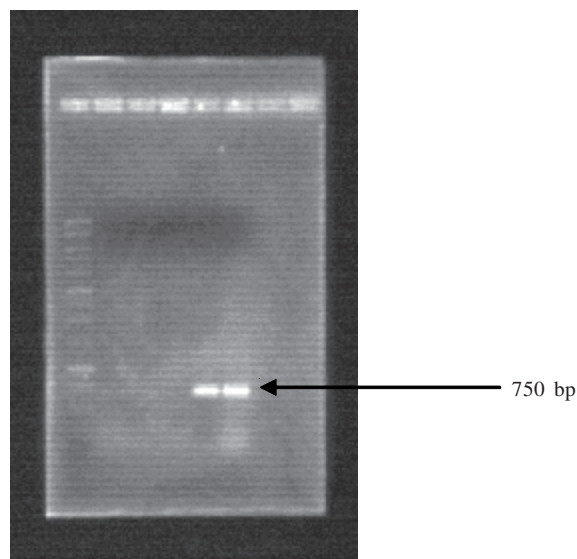
Figure 2 DNA electrophoresis of PCR amplification using specific conserved region class 1 integron (5'CS and 3'CS) primer in 1% (w/v) agarose gel. Well 1 contained DNA marker (1 kb ladder); well 5 contained positive control (PCR amplicon from E. coli origin of Varanus spp.), and well 6 contained PCR amplicon from FC12A isolate (750 bp).
