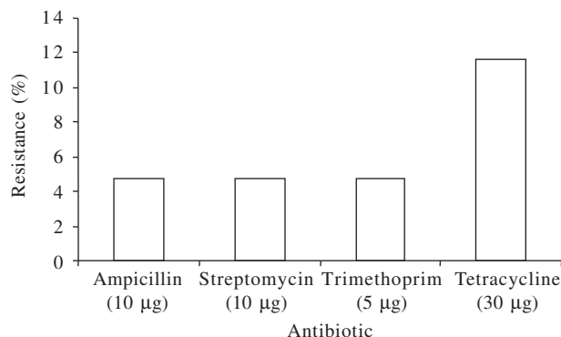
Figure 1 Measurement of resistance by diffusion agar method.
