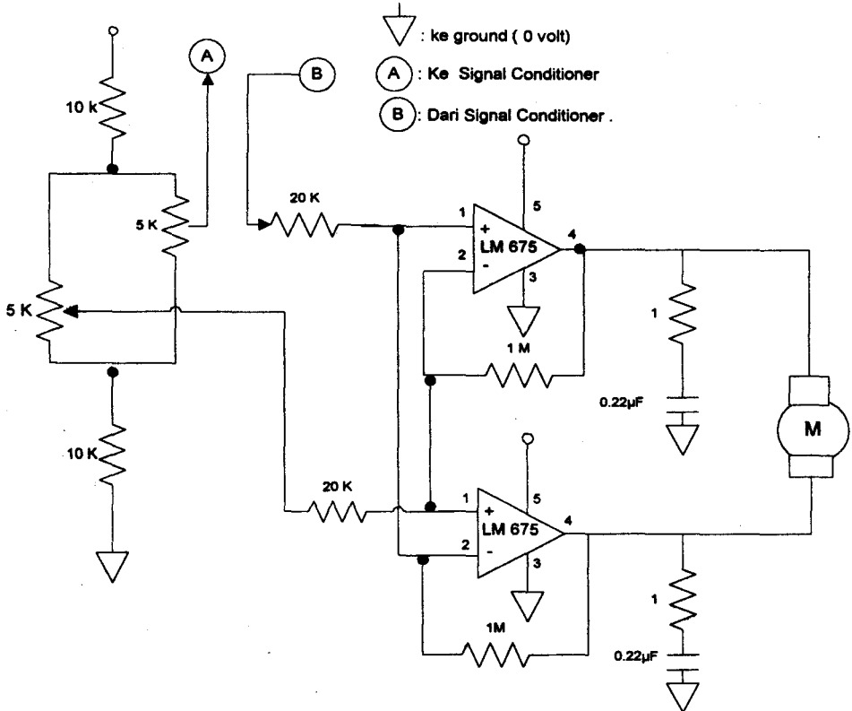
Gambar 4. Driver Motor DC
