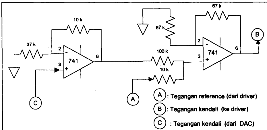
Gambar 3. Signal Conditioner
